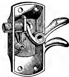
Fig. 4477. Back View. SASH-LOCK.
